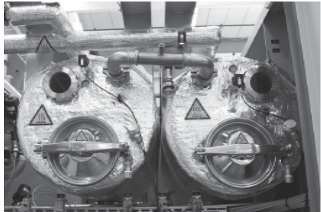
The solvent cleaning plant has two flooding tanks with separate media cycles as a standard. One of these tanks can be used for conservation
